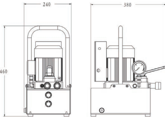
HC Pump
