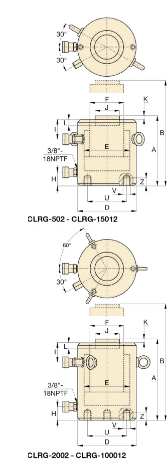
▼ Base Mounting Hole 1) Dimensions (mm)
