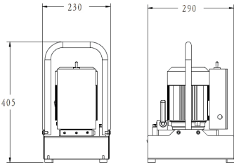
HE Pump
